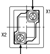
For DC-DC Converter types, terminal X1 is ⊕, X2 is ⊖. Integrated terminal cover
