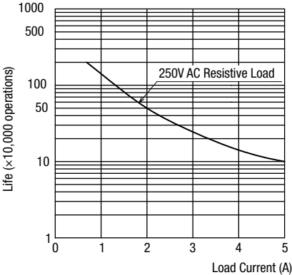
RN2S-NL, RN2S-NF (DPDT)
