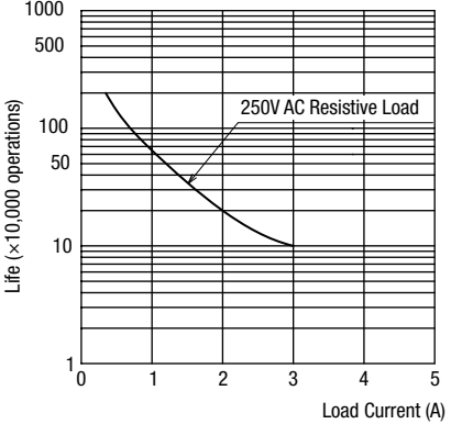
RN4S-NL, RN4S-NF (4PDT)
