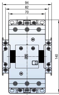
MC-75a-100a AC
