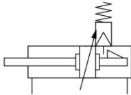
Symbol Air cushion
