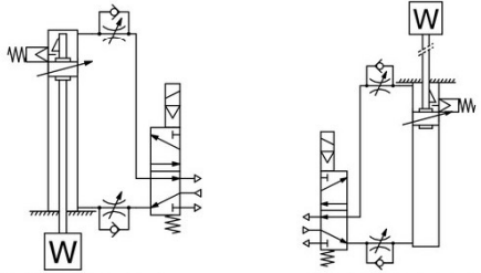
With locking at head end
