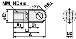
I type Single knuckle joint
