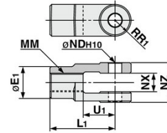
Y type Double knuckle joint
