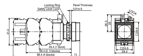
Square Flush (HW2B-M1, -A1)
