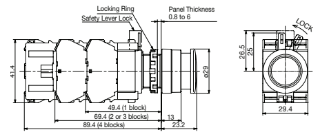
ø29mm Mushroom (HW1B-M3 -A3)
