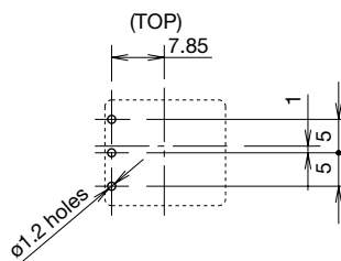
PC Board Terminal Model
