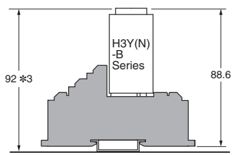
PYF-08-PU-L (PYF-14-PU-L)
