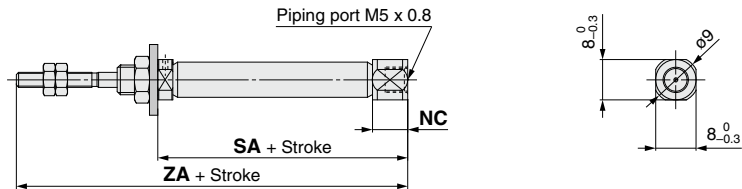
Head cover port location Axial location (R)
