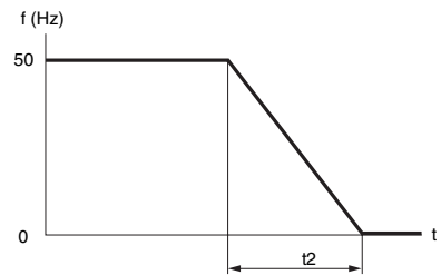
Linear deceleration ramp t1 and t2 can be set independently between 0.1 and 999.9 s. Factory setting: 3 s.
