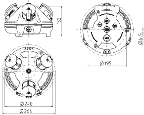
Drawing 1 MB 442 Dim. in mm
